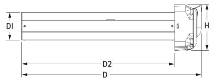
SIDE VIEW
